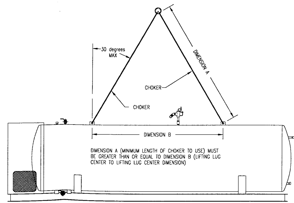
DETAIL LIFTING CHOKERS
